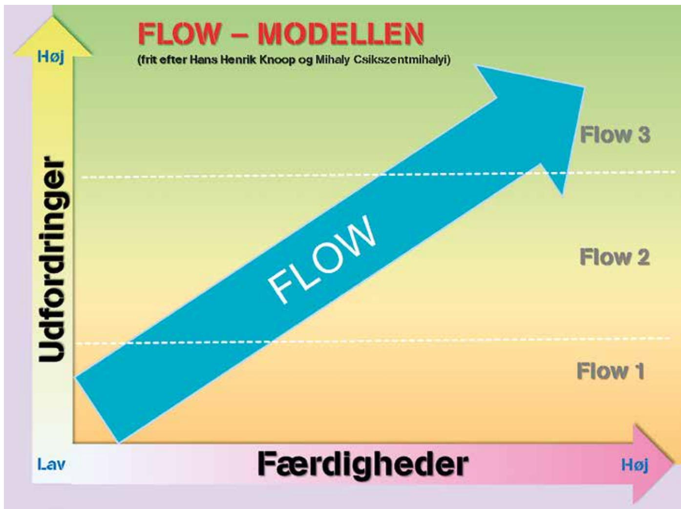
Figur 4: Flow-modellen.
